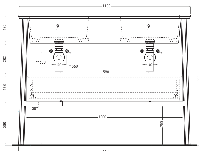
FRONT
