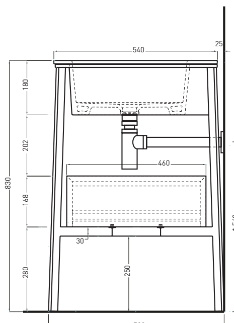
SIDE
