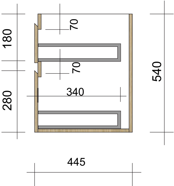
Side Section
