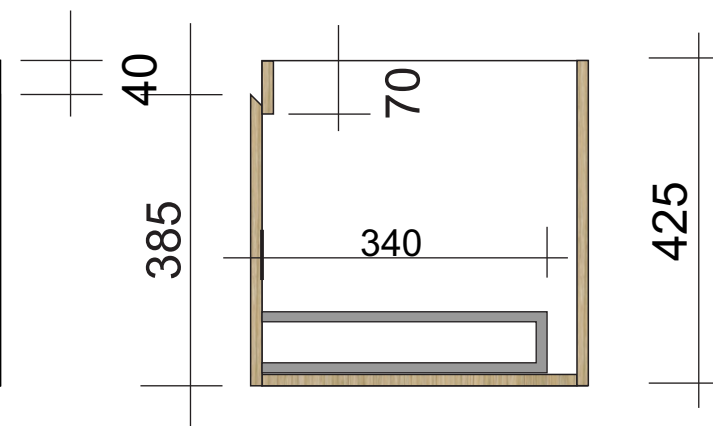
Side Section
