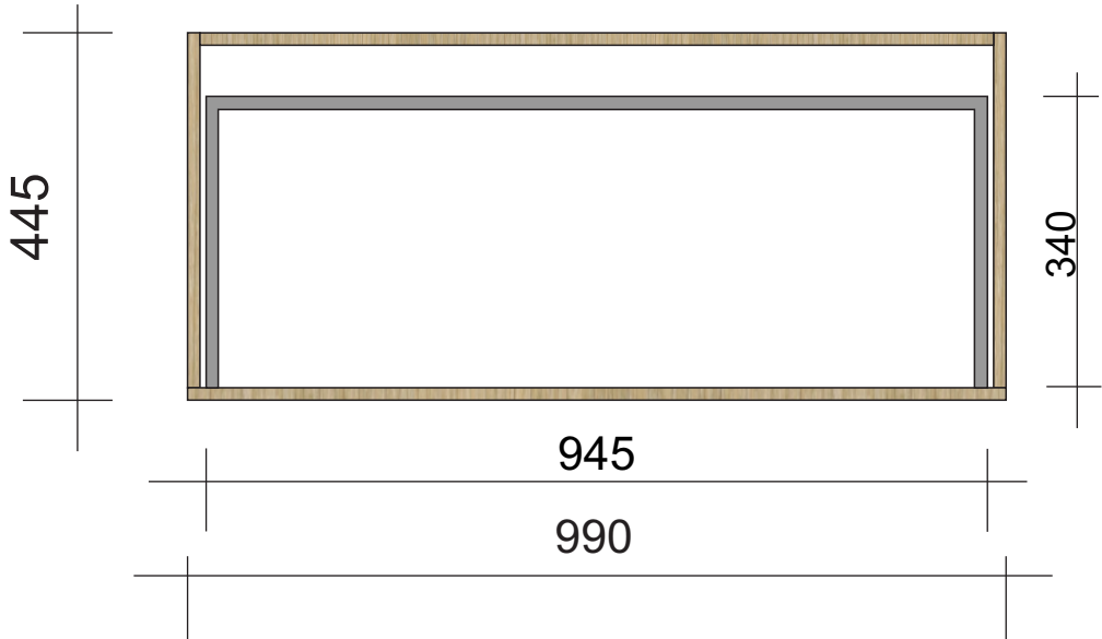
Lower Drawers
