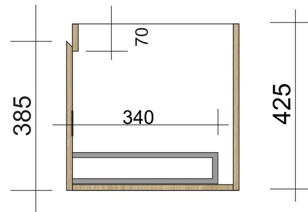
Side Section
