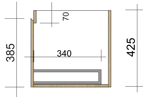
Side Section
