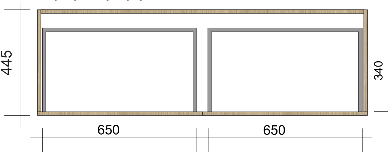
Lower Drawers
