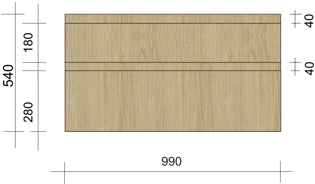
Front Elevation
