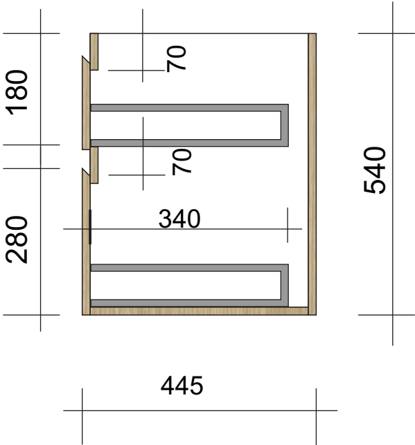
Side Section
